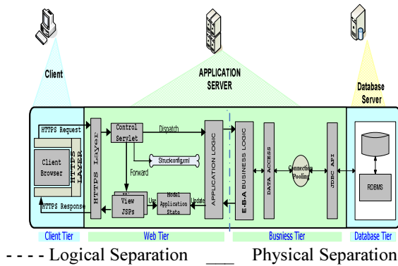
Fig. 2: Vertical Partitioning
