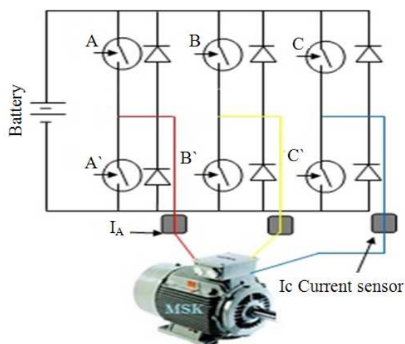
Fig. 1. A six-switch inverter in a three-phase electric drive model
