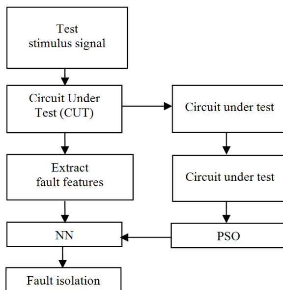
Fig. 2. Flow chart of PSO neural network fault diagnosis
