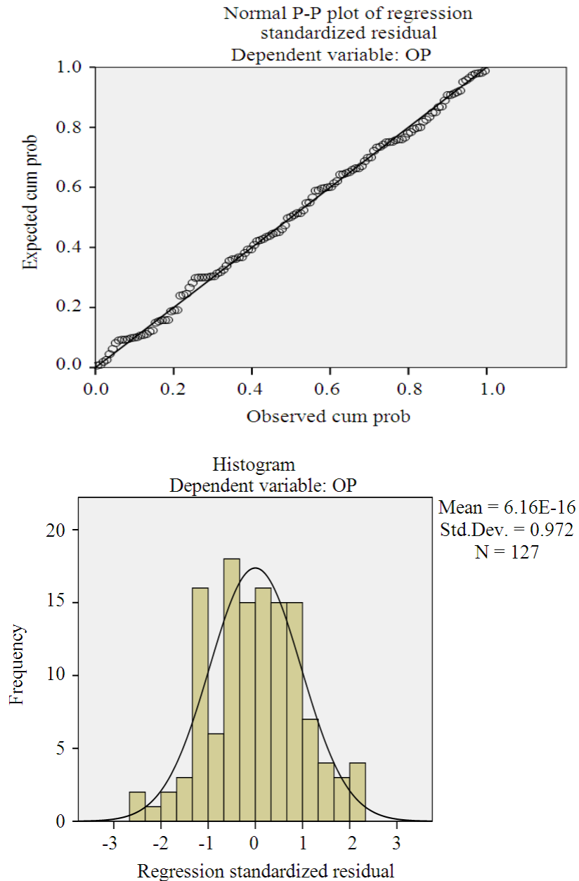
Fig. 2. Model one residual distribution
