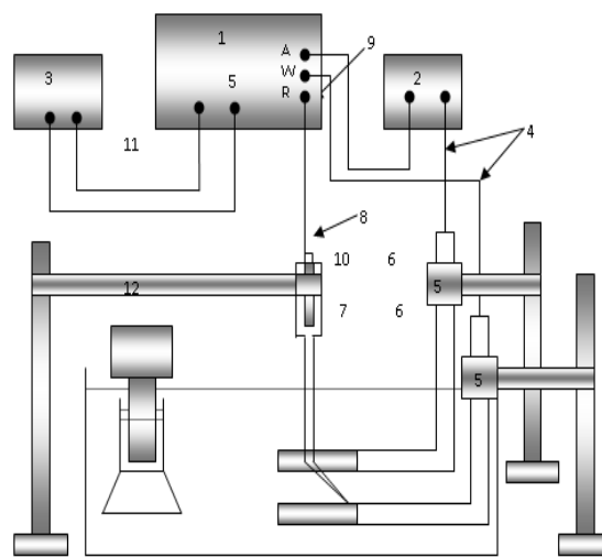
Fig. 1: Experimental setup of cathodic protection (ICCPS), (1) potentiostat; (2) voltmeter; (3) ammeter, (4) connecting wires; (5) stands; (6) pipe plastic; (7) cathode; (8) lugging capillary; (9) Saturated Calomel Electrode (SCE); (10) anode; (11) heater; (12) water bath of distilled water
