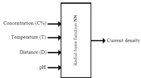
Fig. 2: RBFNN model control
